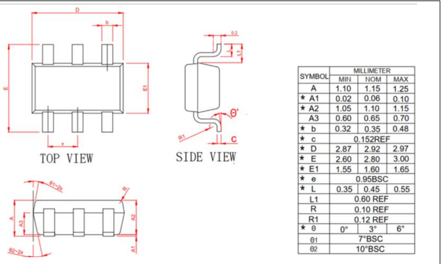
DIMENSIONS, SOT23-6L
