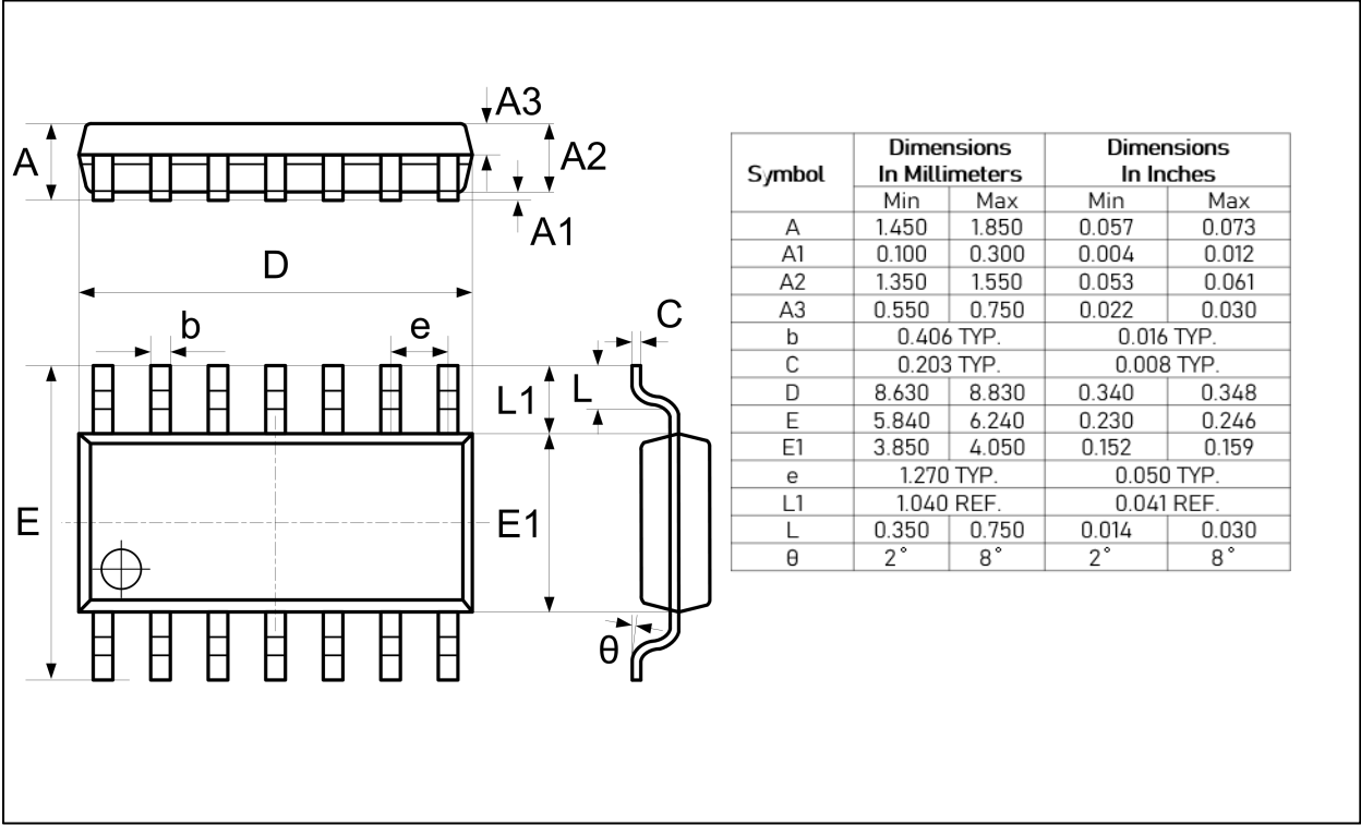
DIMENSIONS, SOIC-14L
