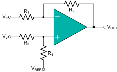
Figure 5. Differential Amplifier
