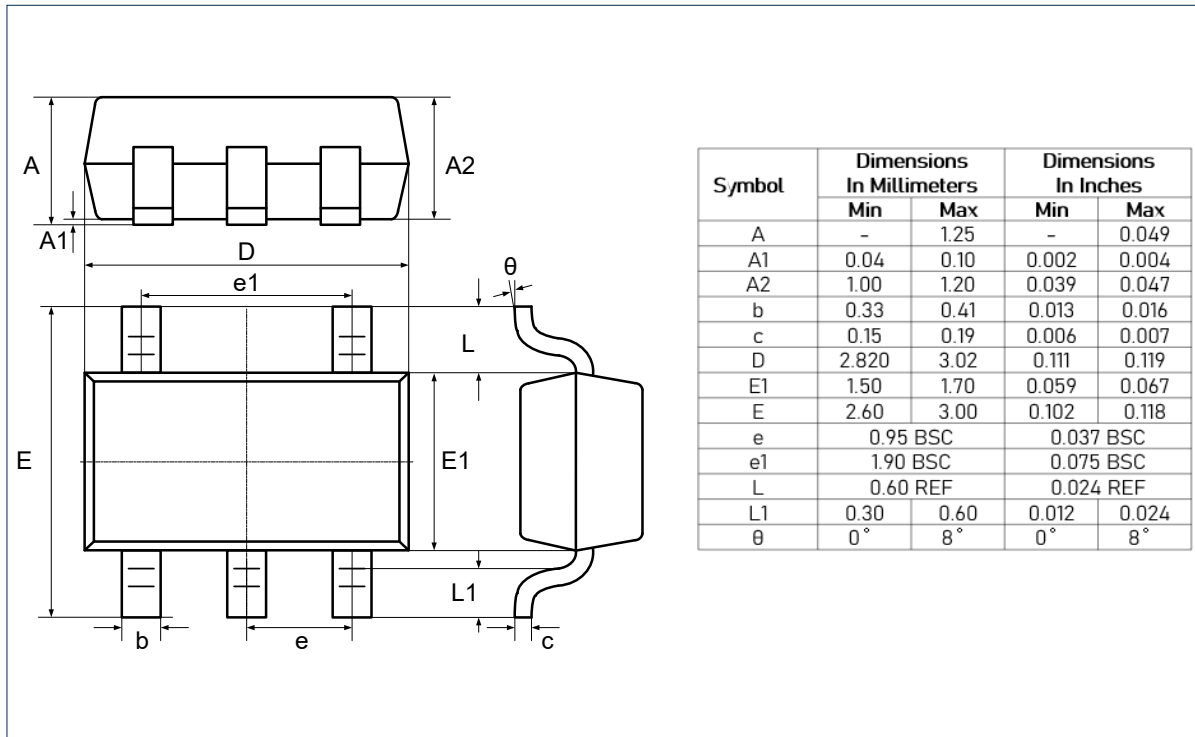
DIMENSIONS, SOT23-5L
