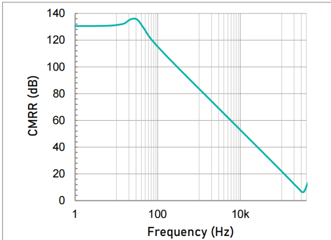
Common-mode Rejection Ratio as a function of Frequency.
