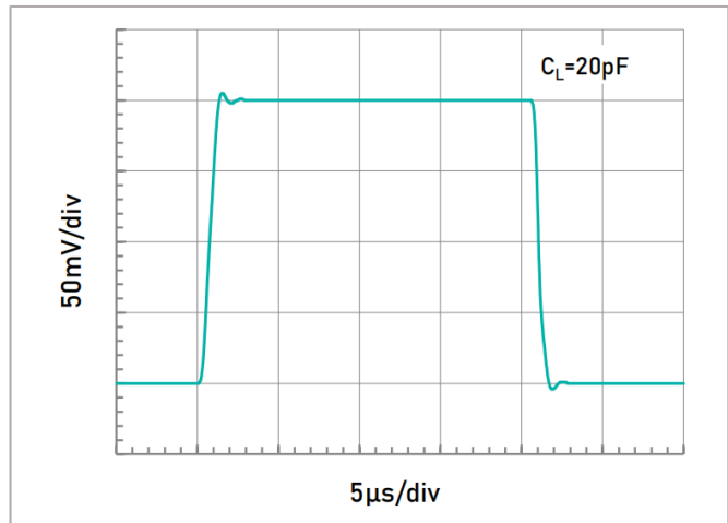
Small Signal Step Response (200mV Step).
