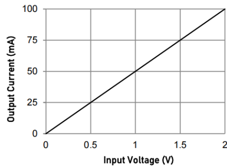
Figure 9. Measured Transfer Function for High-Side V-I Converter
