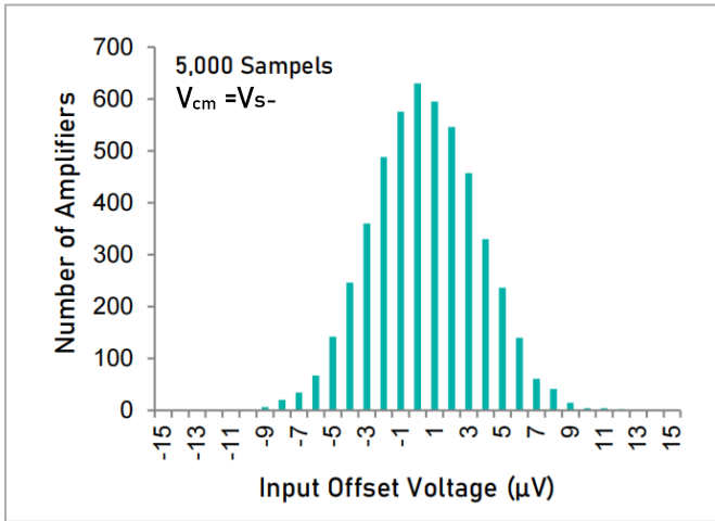
Input Offset Voltage Production Distribution.
