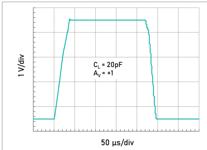
Large Signal Step Response (4V Step).
