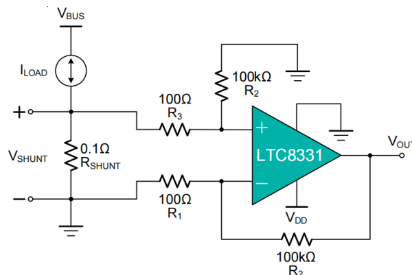
Figure 5: Low-Side Current Sensing Circuit
