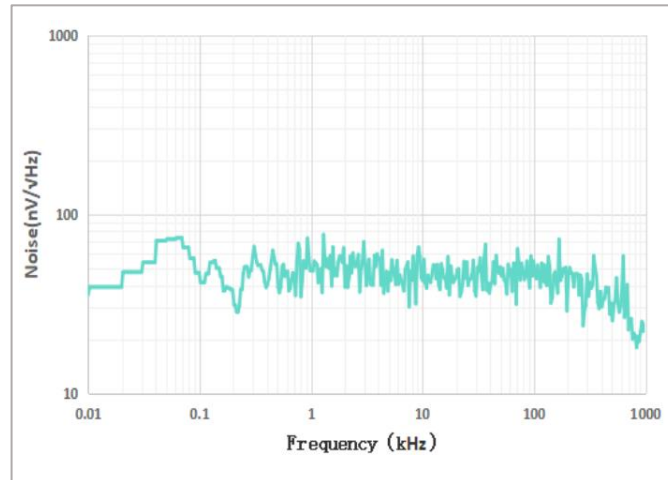
Noise vs. Frequency
