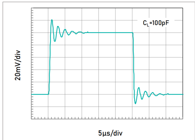
Small Signal Step Response (100mV Step).
