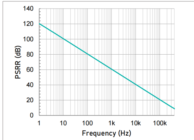
Power Supply Rejection Ratio as a function of Frequency.
