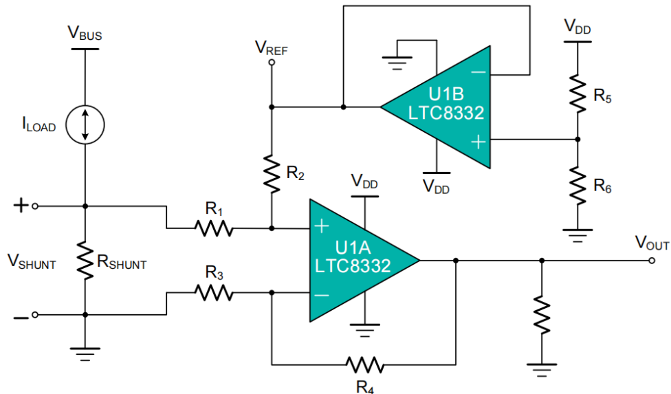
Figure 6. Bidirectional Current-Sensing
