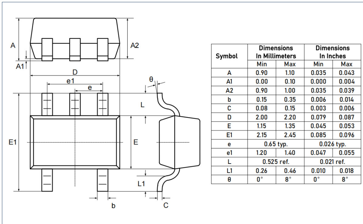
DIMENSIONS, SC70-5L(SOT353)
