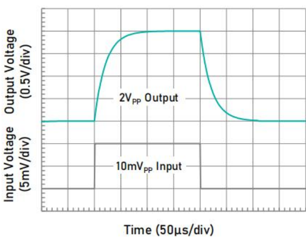
Step Response (10mV pp Input Step)
