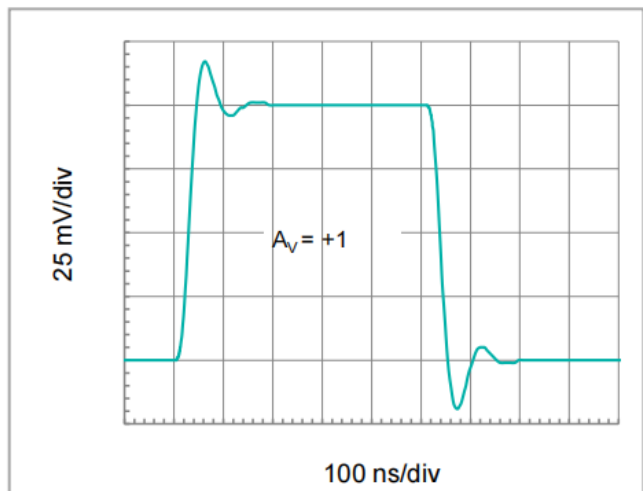
Small Signal Step Response (100mV)
