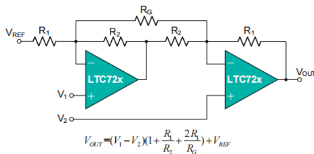
Figure 9: Instrumentation Amplifier
