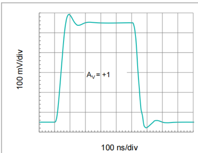
Small Signal Step Response (500mV)
