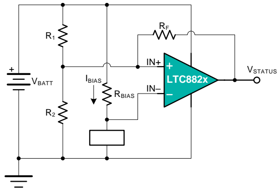
Figure 7. Battery Monitor
