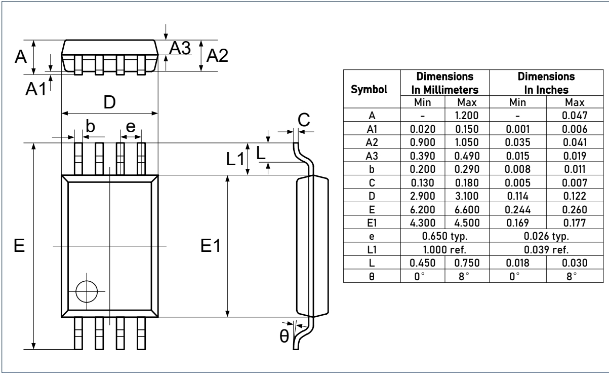
DIMENSIONS, TSSOP-8L
