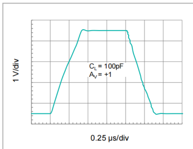
Large Signal Step Response.
