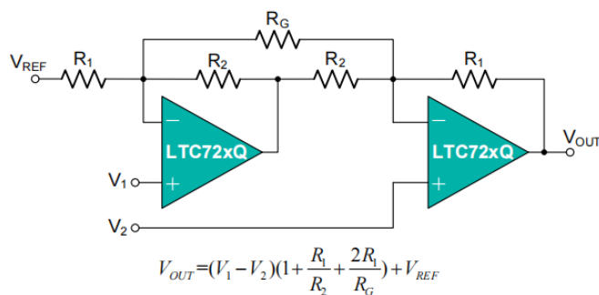
Figure 9: Instrumentation Amplifier
