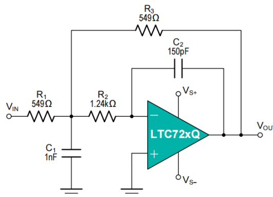
Figure 5: Second-Order, Butterworth, 500-kHz Low-Pass Filter
