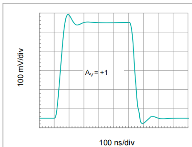
Small Signal Step Response (500mV)
