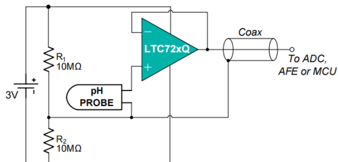
Figure 10: Buffered pH Probe
