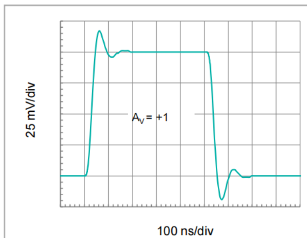
Small Signal Step Response (100mV)
