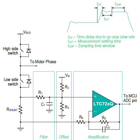
Figure 7: Current Shunt Monitor Circuit
