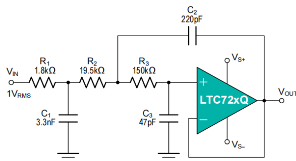
Figure 6: Configure as a Three-Pole, 20-kHz, Sallen-Key Filter
