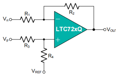
Figure 8: Differential Amplifier
