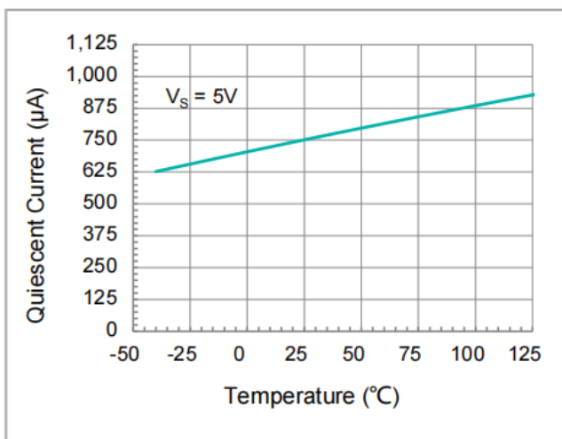
Quiescent Current as a function of Temperature.
