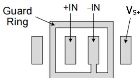
Figure 4: Use a guard ring around sensitive pins
