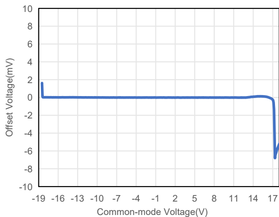
Offset Voltage vs Common-mode Voltage ( V_S = 36\text{ V} )
