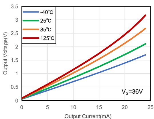
Output Voltage Swing as a function of Output Current (Sinking, V_S = 36\text{ V} )
