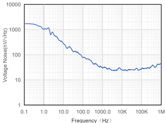
Voltage Noise Density vs. Frequency
