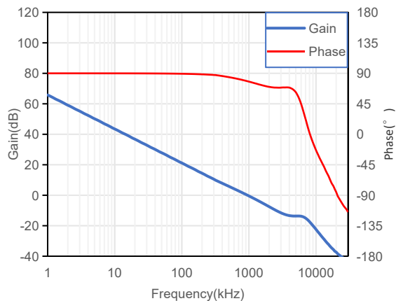
Open-Loop Gain and Phase vs. Frequency
