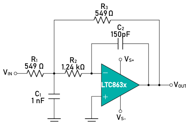
Figure 5: Second-Order, Butterworth, 500-kHz Low-Pass Filter
