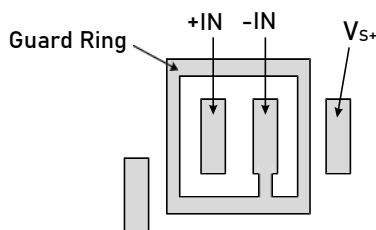
Figure 4: Use a guard ring around sensitive pins
