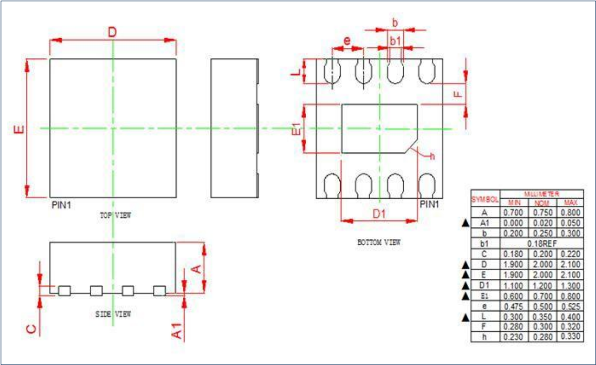
DIMENSIONS, DFN2x2-8L
