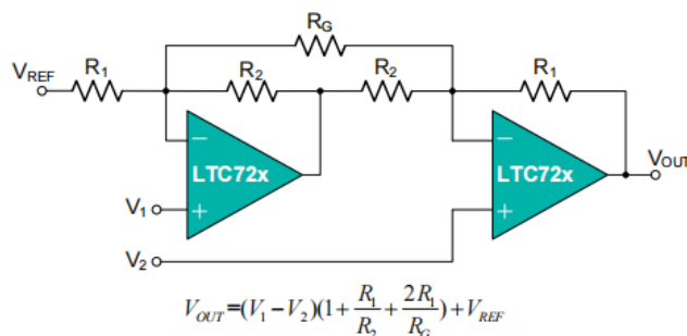
Figure 9: Instrumentation Amplifier
