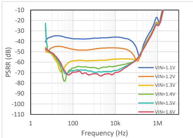
Figure 9. PSRR vs Frequency for Various input voltage, V_{OUT} = 0.9\text{ V} , Load current = 3 A
