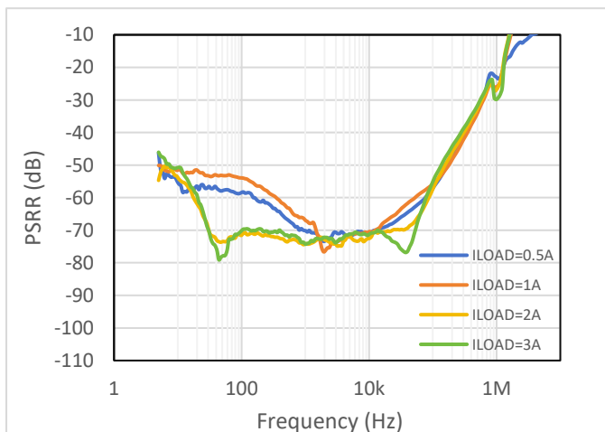
Figure 11. PSRR vs Frequency for Various loads, V_{OUT} = 1.3\text{ V} , V_{OUT} = 1.7\text{ V}
