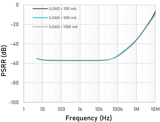
Figure 33. Power supply rejection ratio vs Frequency (1.2 V Adjustable version & V_{out} = 5\text{ V} , 500mV headroom )
