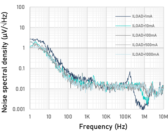
Figure 39. Output noise spectral density vs Frequency (Adjustable version Vout = 1.2 V)
