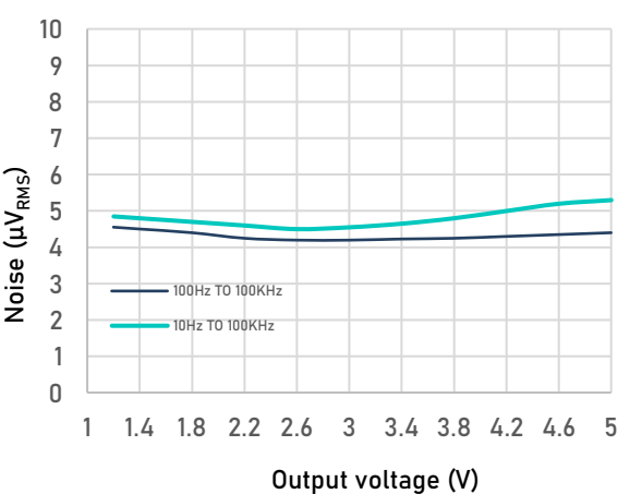
Figure 38. RMS Output Noise vs Output voltage (Load current = 100 mA)
