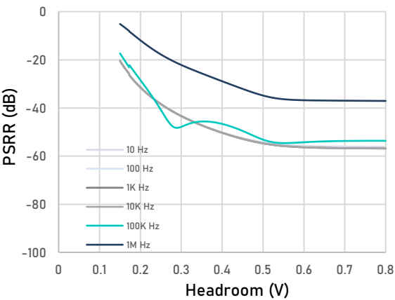
Figure 31. Power supply rejection ratio vs Headroom (1.2 V Adjustable version & V_{out} = 5\text{ V} , 2A load current, Different Frequencies )
