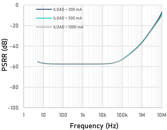
Figure 32. Power supply rejection ratio vs Frequency (1.2 V Adjustable version & V_{out} = 5\text{ V} , 800mV headroom )
