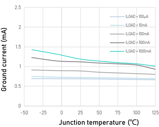
Figure 22. Ground current vs Junction temperature Adjustable version (Vout = 1.2 V)
