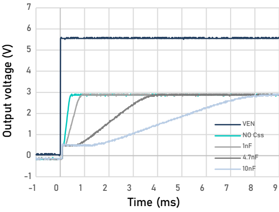
Figure 44. Typical soft start behavior, Different Ccss values
