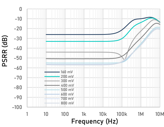
Figure 26. Power supply rejection ratio vs Frequency (Vout = 3 V, 2A load current, Various headroom voltages )
