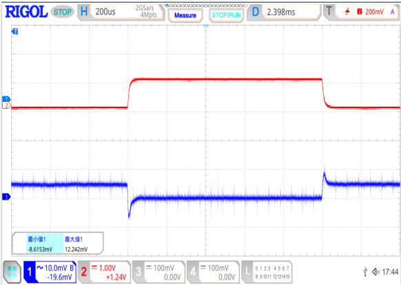
Figure 45. Load Transient Response, I_{LOAD} = 10\text{ mA} to 1\text{ A} , 1.2\text{ V} Adjustable version & V_{out} = 5\text{ V} , V_{IN} = 5.5\text{ V} , CH1 = V_{OUT} , CH2 = I_{LOAD}
