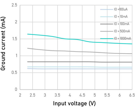
Figure 24. Ground current vs Input voltage Adjustable version (Vout = 1.2 V)
