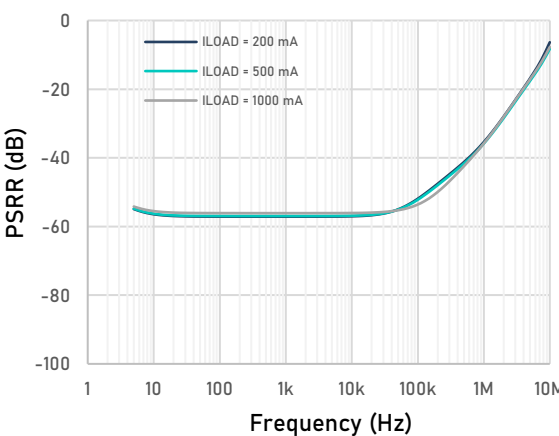
Figure 34. Power supply rejection ratio vs Frequency (1.2 V Adjustable version & V_{out} = 5\text{ V} , 400mV headroom )
