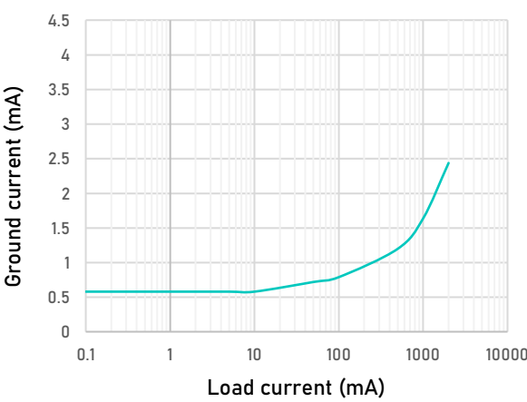
Figure 23. Ground current vs Load current Adjustable version (Vout = 1.2 V)
