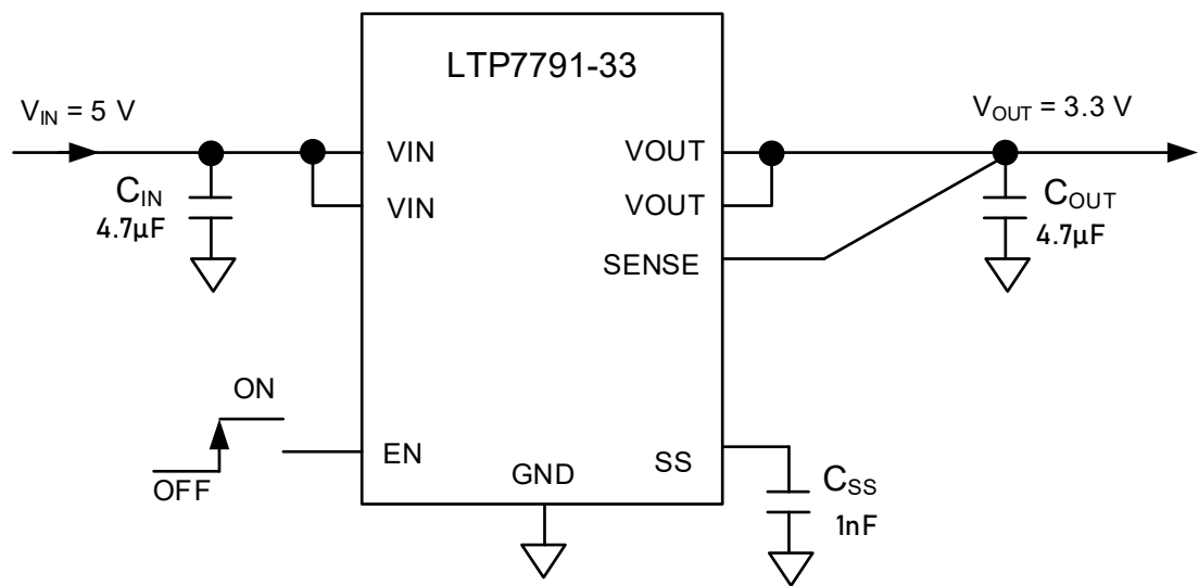
Fixed Output Voltage, 3.3 V
