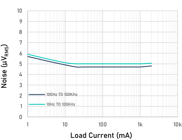
Figure 37. RMS Output Noise vs Load Current (1.2 V Adjustable version & Vout = 5 V)
