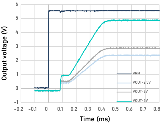
Figure 43. Typical start-up behavior
