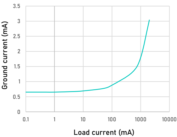
Figure 14. Ground current vs Load current (Vout = 3 V)
