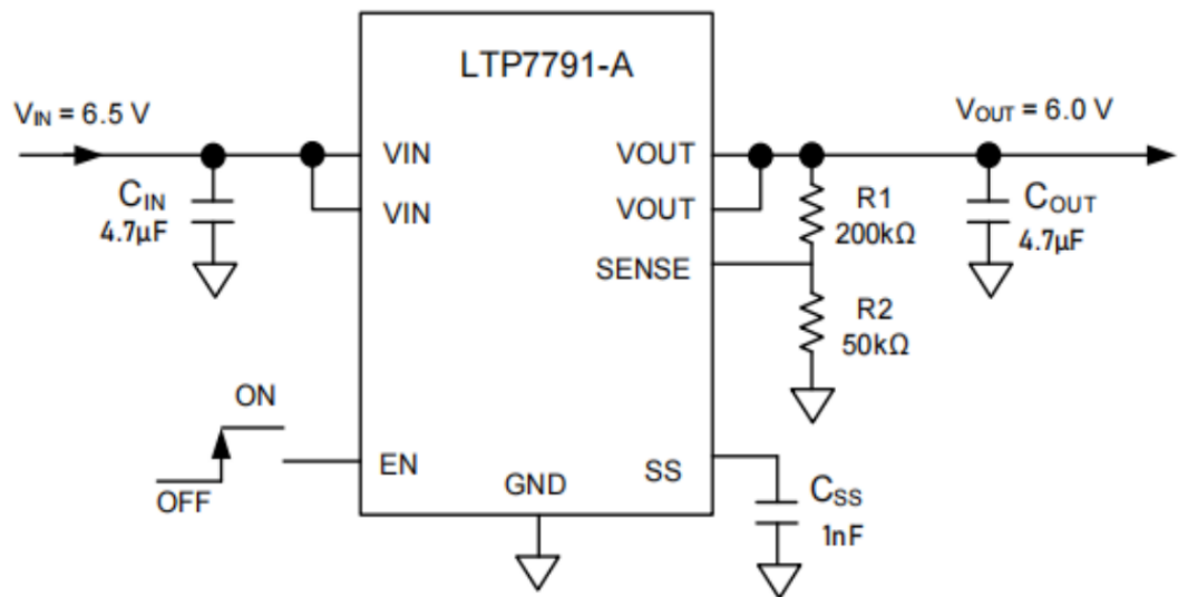
Adjustable Output Voltage Application with Adjustable Output Version LTP7791-A: V_{OUT} = 1.2\text{V} \cdot (1 + R1/R2)
