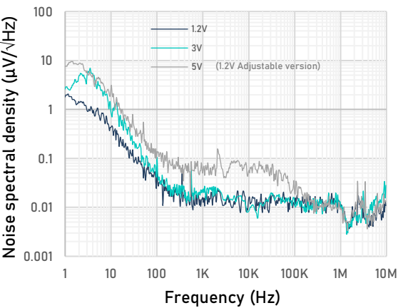
Figure 42. Output noise spectral density vs Frequency (Different output voltages, I LOAD = 100 mA)
