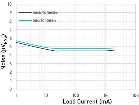
Figure 35. RMS Output Noise vs Load Current (Adjustable version V_{out} = 1.2\text{ V} )
