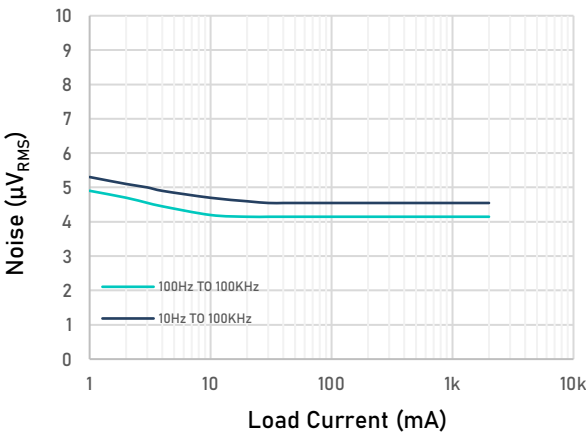
Figure 36. RMS Output Noise vs Load Current ( V_{out} = 3\text{ V} )
