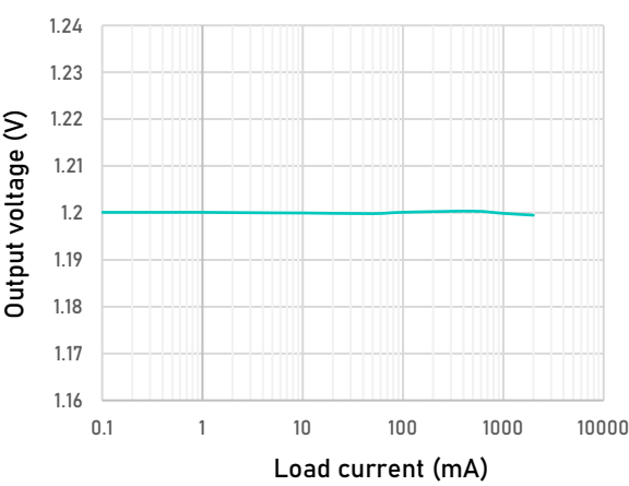
Figure 20. Output voltage vs Load current Adjustable version (Vout = 1.2 V)
