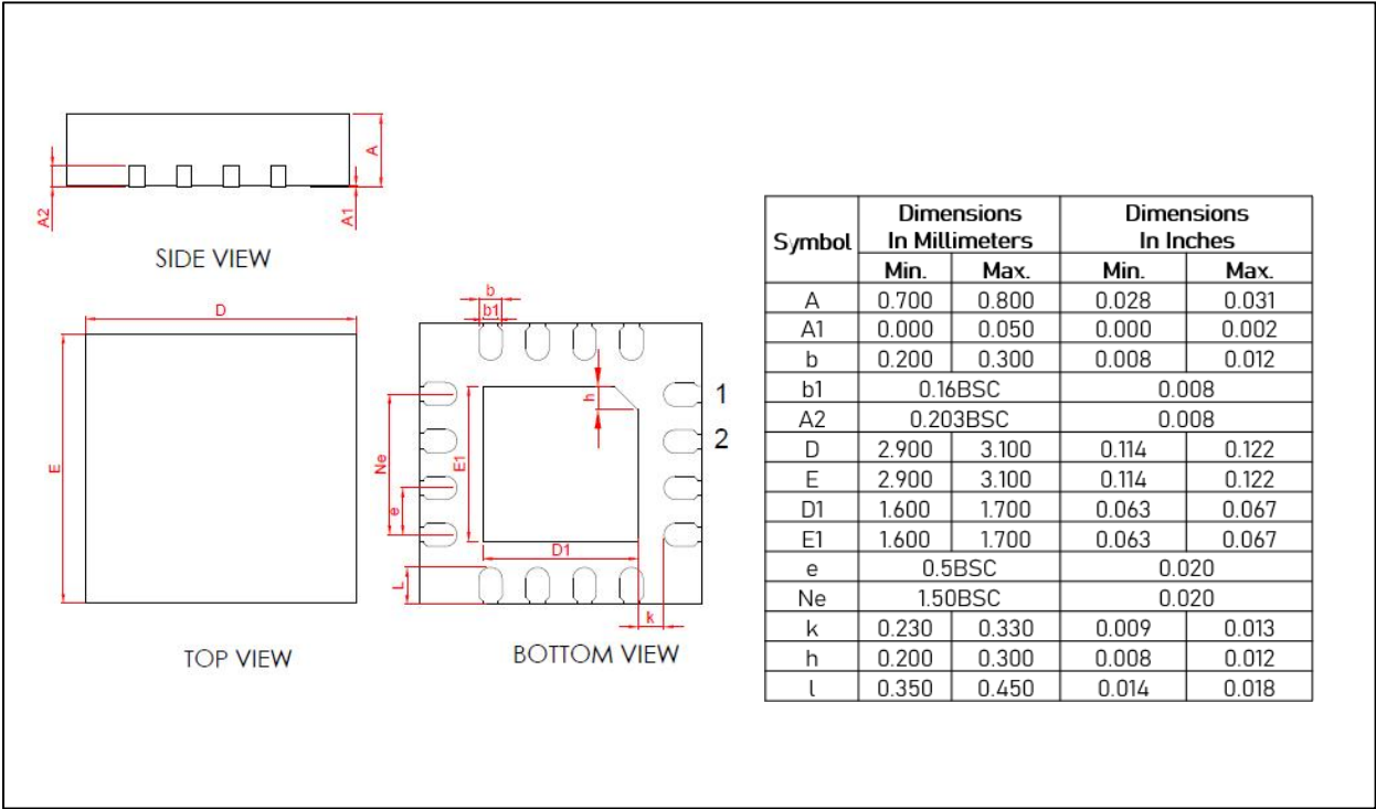
DIMENSIONS, QFN 3x3-16L
