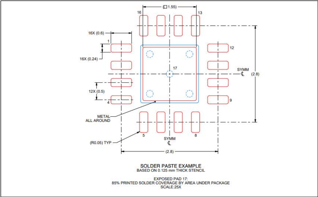
RECOMMENDED SOLDERING FOOTPRINT, QFN 3x3-16L
