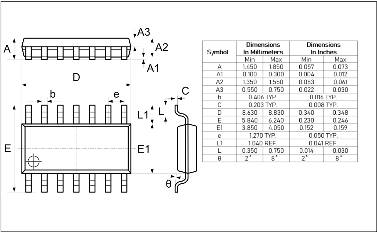
DIMENSIONS, SOIC-14L
