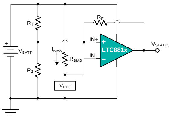
Figure 7. Battery Monitor
