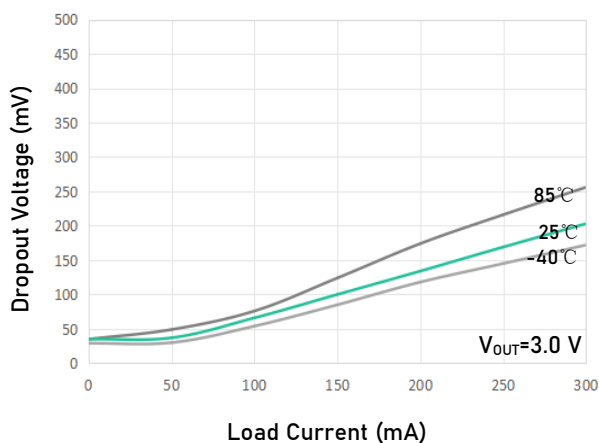
Dropout Voltage vs. Load Current V_{OUT} = 3.0 \text{ V DFN1} \times 1\text{-}4\text{L}
