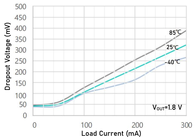
Dropout Voltage vs. Load Current V_{OUT} = 1.8 \text{ V DFN2} \times 2\text{-}6\text{L}
