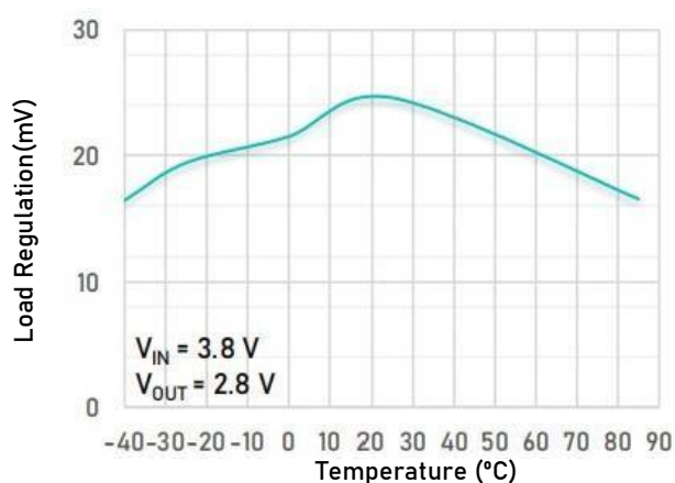
Load Regulation vs. Temperature
