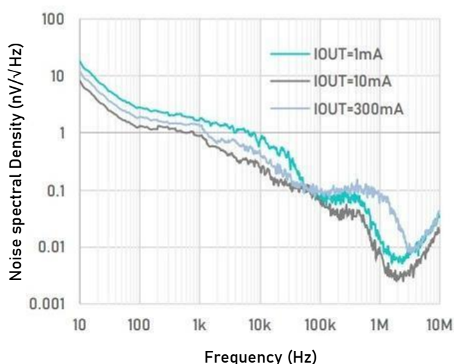
Output Voltage Noise Spectral Density vs. Frequency
