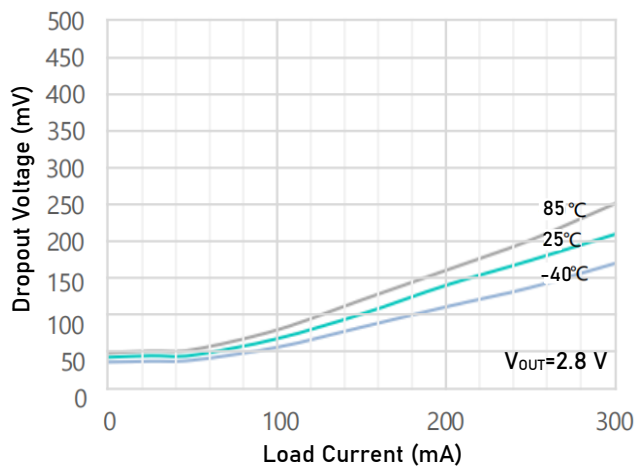
Dropout Voltage vs. Load Current V_{OUT} = 2.8 \text{ V DFN1} \times 1\text{-}4\text{L}
