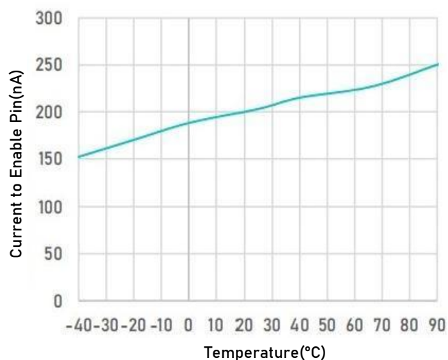
Current to Enable Pin vs. Temperature
