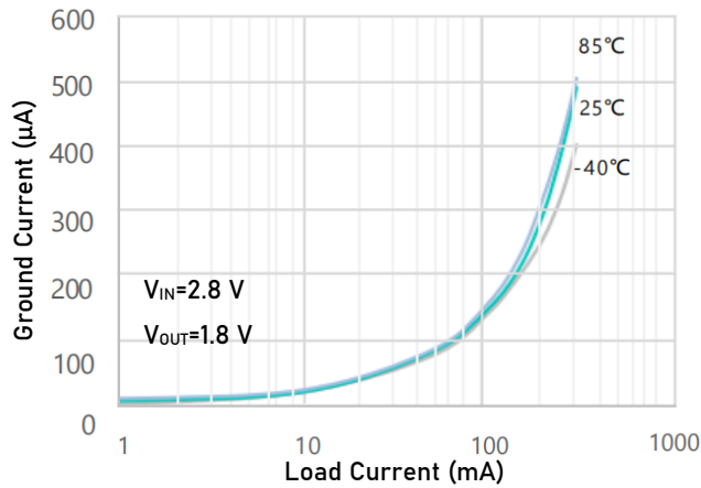
Ground Current vs. Load Current V_{OUT} = 1.8 \text{ V DFN2} \times 2\text{-}6\text{L}
