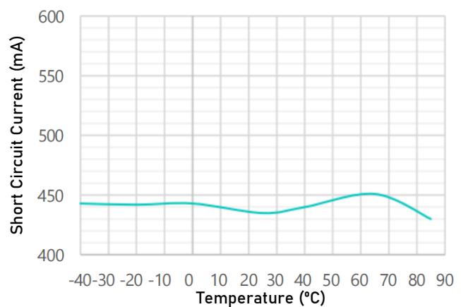
Short Circuit Current vs. Temperature V_{OUT} = 1.8 \text{ V DFN2} \times 2\text{-}6\text{L}
