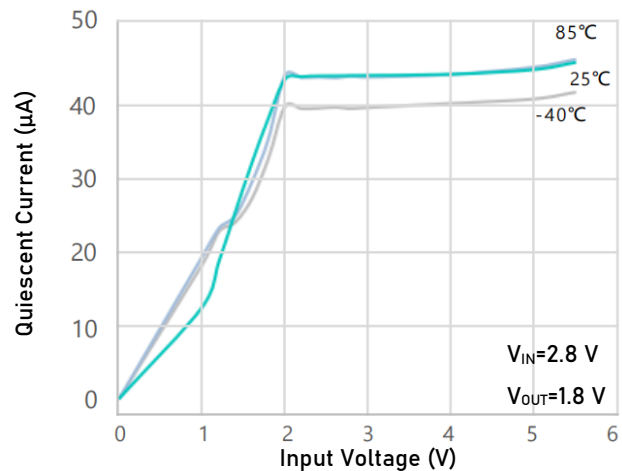
Quiescent Current vs. Input Voltage V_{OUT} = 1.8 \text{ V DFN2} \times 2\text{-}6\text{L}
