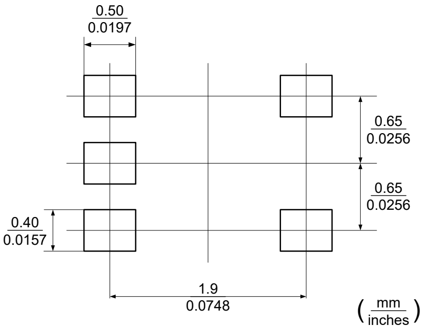
RECOMMENDED SOLDERING FOOTPRINT, SC70-5L (SOT353)
