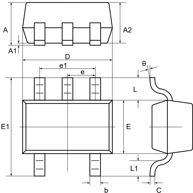
DIMENSIONS, SC70-5L (SOT353)
