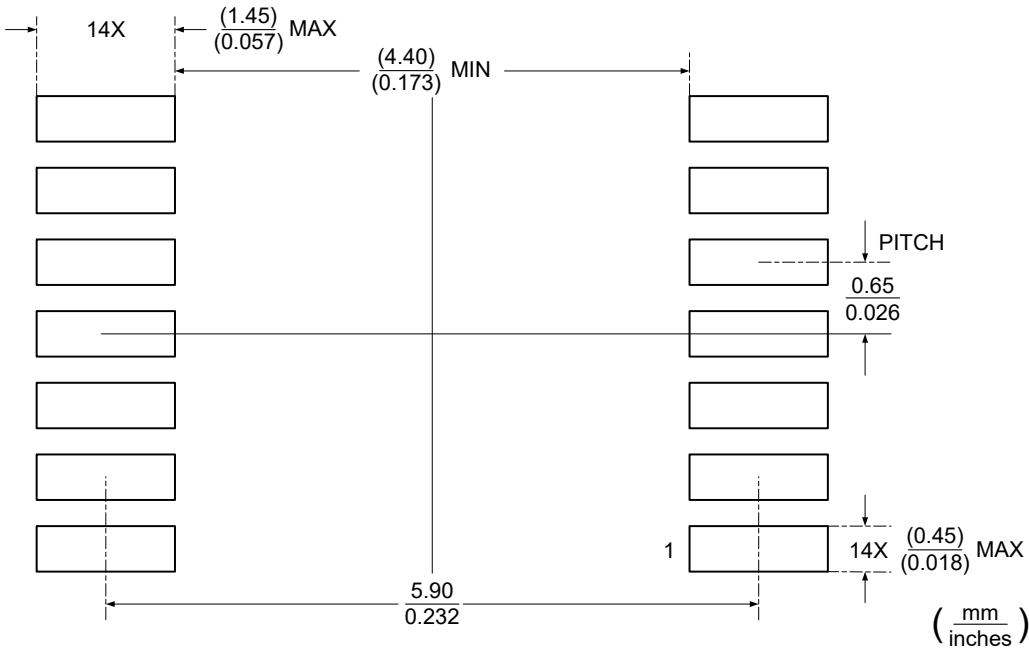
RECOMMENDED SOLDERING FOOTPRINT, TSSOP-14L
