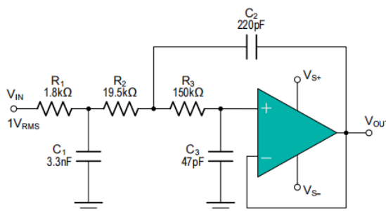
Figure 6: Configure as a Three-Pole, 20-kHz, Sallen-Key Filter
