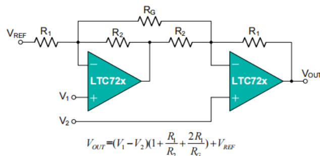
Figure 9: Instrumentation Amplifier
