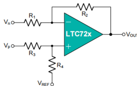
Figure 8: Differential Amplifier
