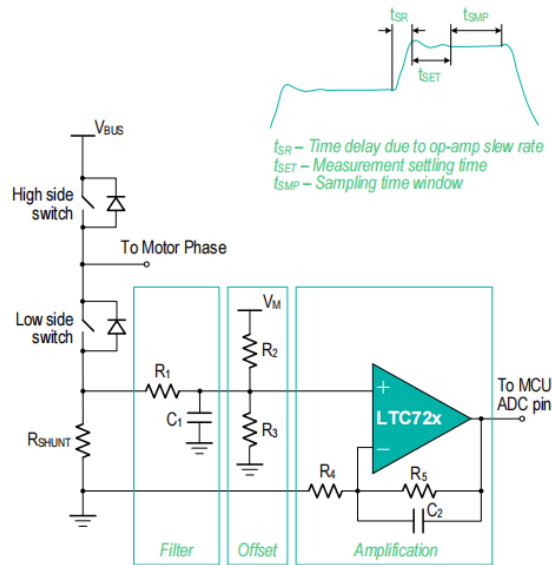
Figure 7: Current Shunt Monitor Circuit
