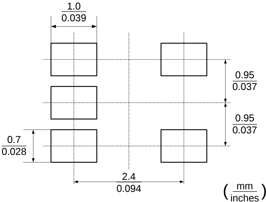
RECOMMENDED SOLDERING FOOTPRINT, SOT23-5L
