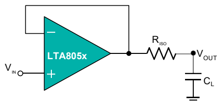
Figure 1. Indirectly Driving Heavy Capacitive Load
