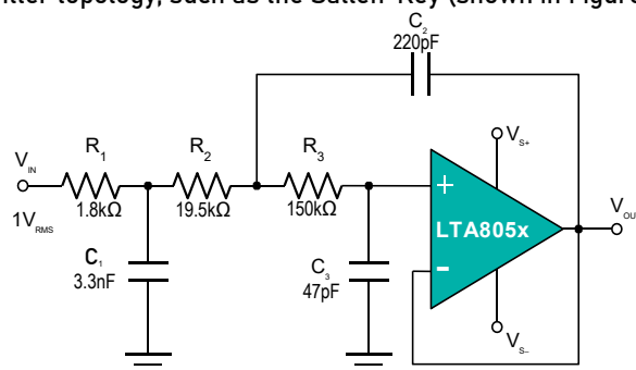
Figure 4. Configured as a Three-Pole, 20-kHz, Sallen-Key Filter
