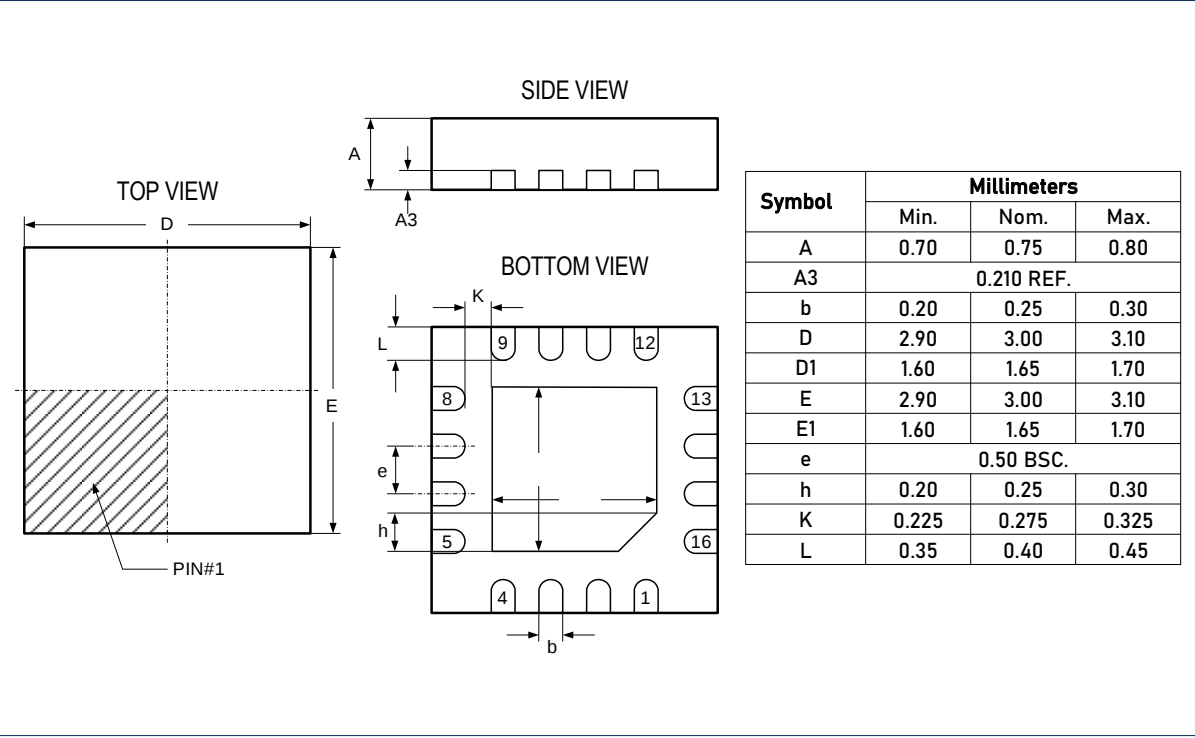
DIMENSIONS, QFN3x3-16L
