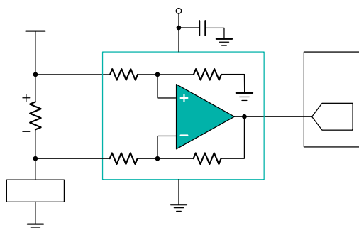
Figure 1. Typical Application
