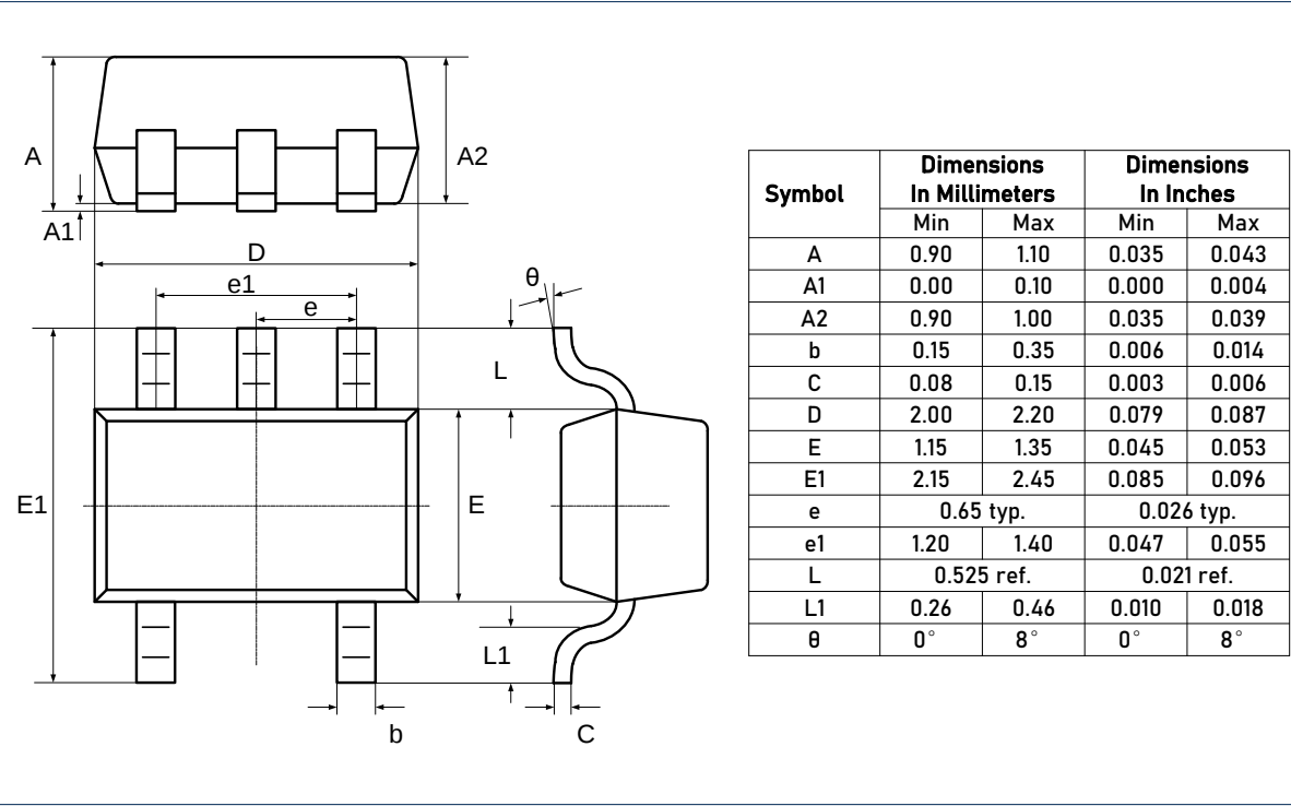
DIMENSIONS, SC70-5L (SOT353)
