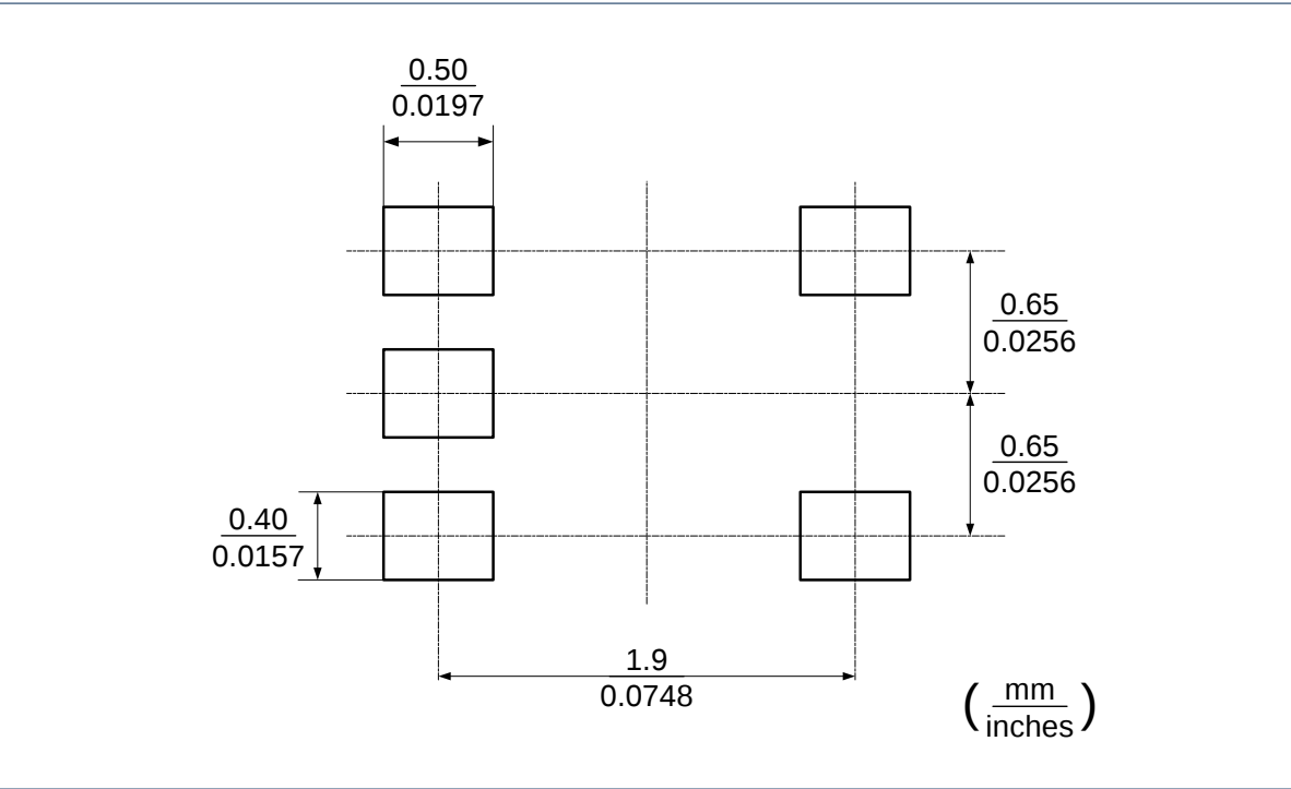
RECOMMENDED SOLDERING FOOTPRINT, SC70-5L (SOT353)
